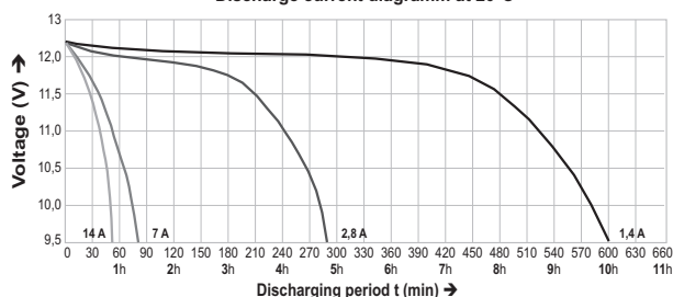
Discharge current diagram at 20°C
